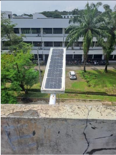
Solar Panel found in the Main Administration Building, Solar panel in Faculty of Engineering integrated Lab ,Class Room, Solar-powered lights along at Universitas Street and Solar charging at shuttle bus
